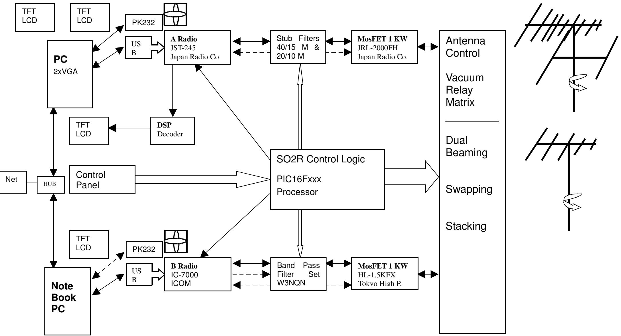
OH2BP SO2R 2007 CONCEPT / Cushcraft X9 9 el & XM240 + Fritzel 5 el + sloopers
