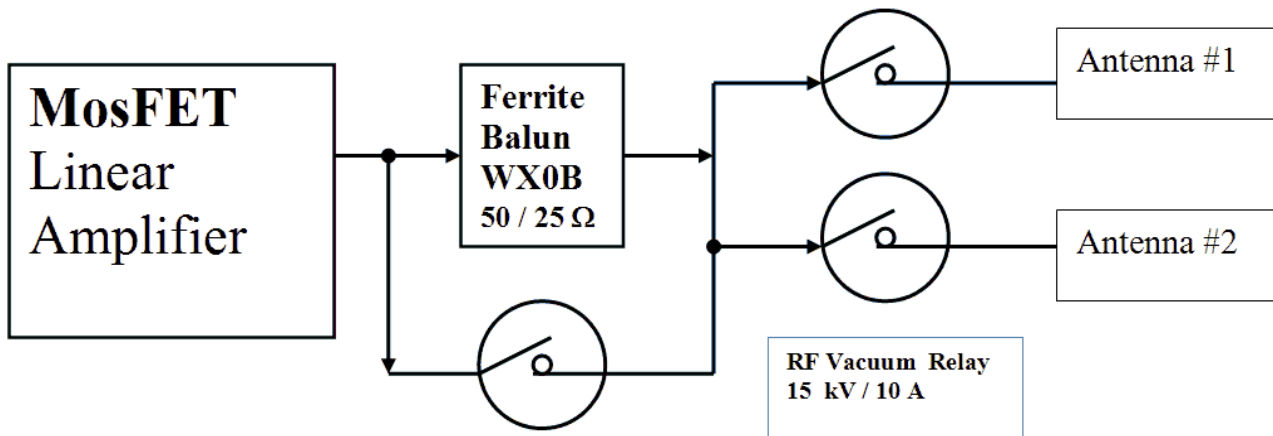
Drawing 2. Principle of stacking.
